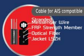
FTTH-01SM9 1 cores SM FTTH-02SM9 2 cores SM FTTH-04SM9 4 cores SM
