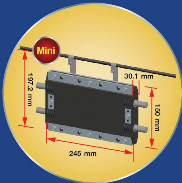
CL002 Fiber Closure 24 cores
